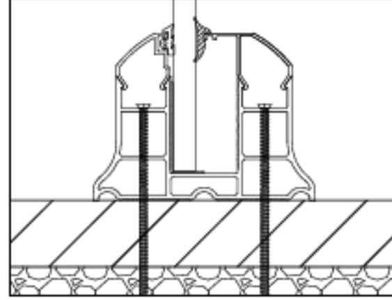
ALT BAZA DETAYI LOWER BASE FEATURE
