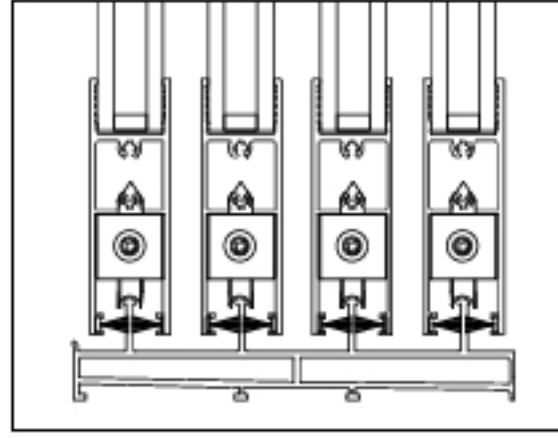
4'lü Eşikli Ray Sistemi Quadruple Lifted Rail System
